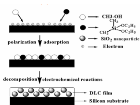
Schematic of the two steps involved in the growth of carbon/silica nanocomposite film
