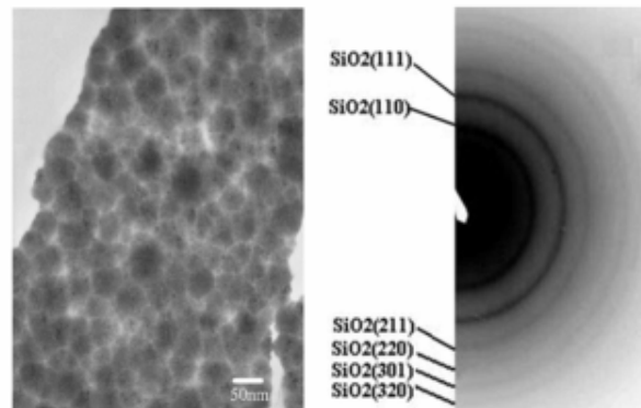
TEM image and electron diffraction pattern of the carbon/silica nanocomposite film
